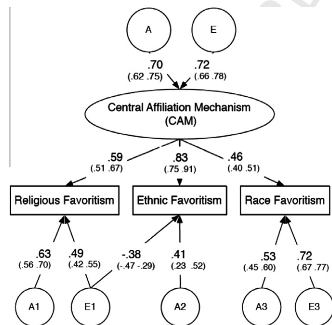
Fig. 2. Common pathway model as a test of two theories of in-group favoritism (from Lewis & Bates, 2010).
